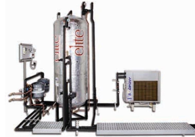
SOLARIZER ELITE HYBRID Provides bulk hot water 24/7
